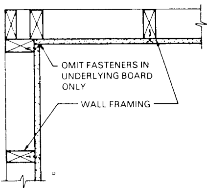
FIG. 13 Horizontal Section Through Interior Vertical Angle
